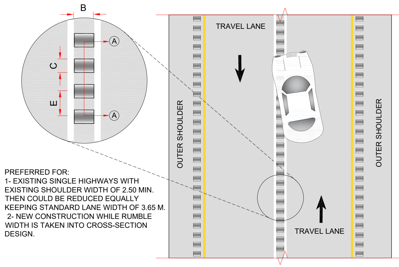
FIGURE (2): CENTER LINE RUMBLE STRIPS PATTERN ON SINGLE HIGHWAY (CONTINUOUS APPLICATION) N.T.S
