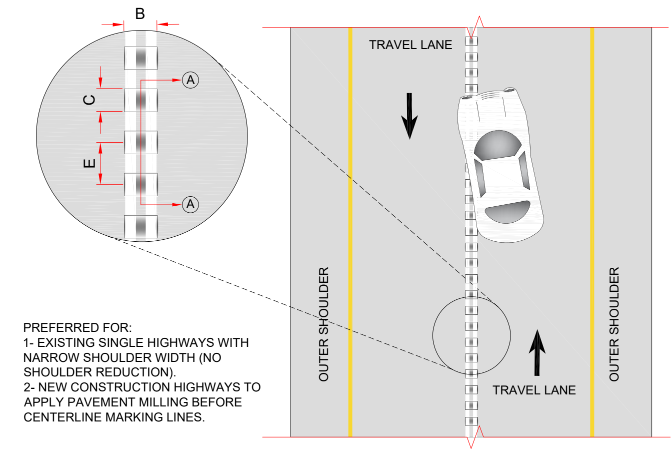
FIGURE (6): CENTER LINE RUMBLE STRIPES PATTERN ON SINGLE HIGHWAY (CONTINUOUS APPLICATION) N.T.S
