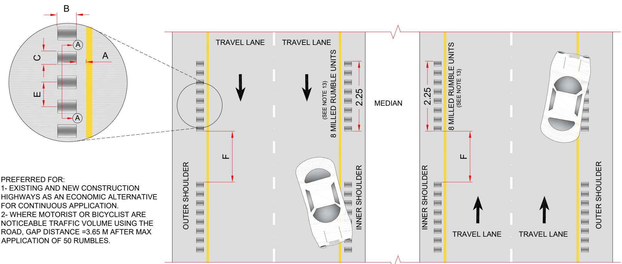
FIGURE (3): TYPICAL APPLICATION PATTERN OF RUMBLES WITH GAP DISTANCE ON DIVIDED & SINGLE HIGHWAY SHOULDERS (APPLICABLE FOR RUMBLE STRIPS & RUMBLE STRIPES TYPES) N.T.S
