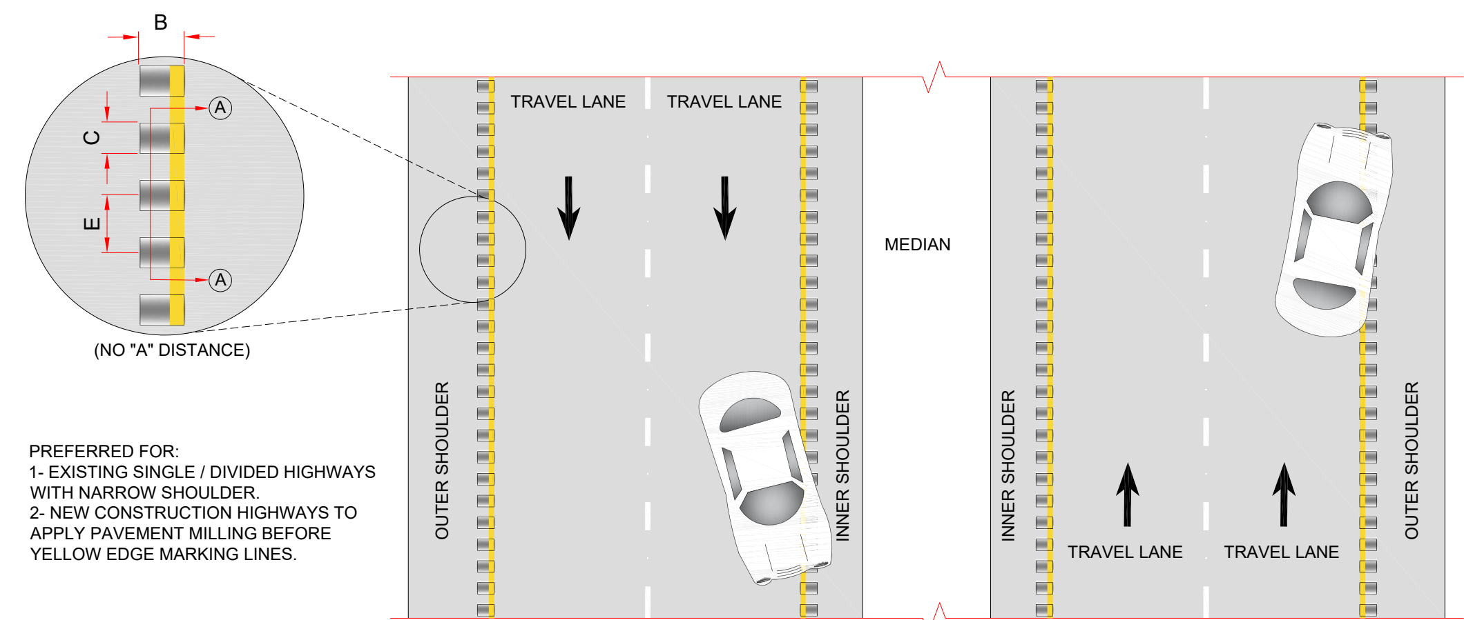
FIGURE (5): SHOULDER RUMBLE STRIPES PATTERN ON DIVIDED & SINGLE HIGHWAYS (CONTINUOUS APPLICATION) N.T.S
