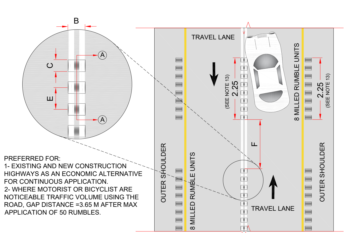
FIGURE (4): TYPICAL APPLICATION PATTERN OF RUMBLES WITH GAP DISTANCE ON SINGLE HIGHWAY CENTERLINE (APPLICABLE FOR RUMBLE STRIPS & RUMBLE STRIPES TYPES) N.T.S
