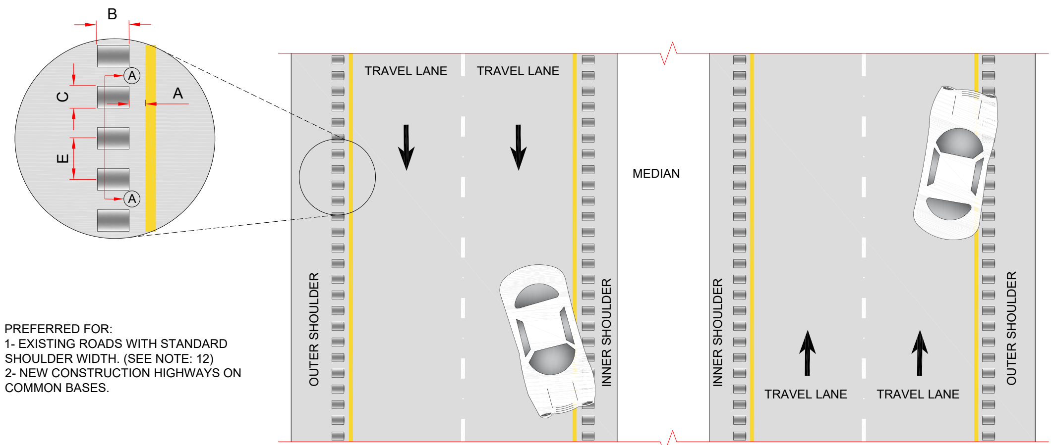
FIGURE (1): SHOULDER RUMBLE STRIPS PATTERN ON DIVIDED & SINGLE HIGHWAYS (CONTINUOUS APPLICATION) N.T.S
